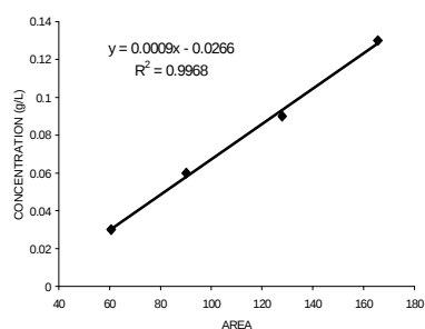
Figure 5. Calibration curve of the indirubin.
